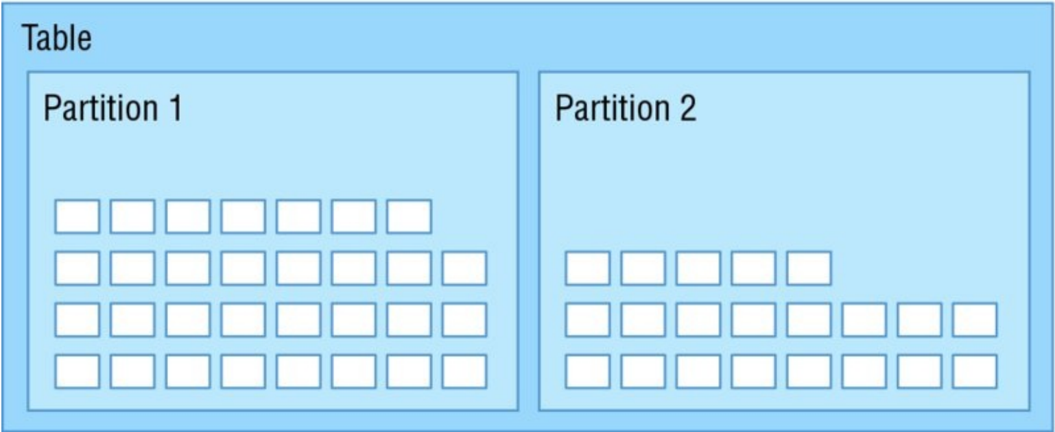
FIGURE 7.4 Table partitioning
